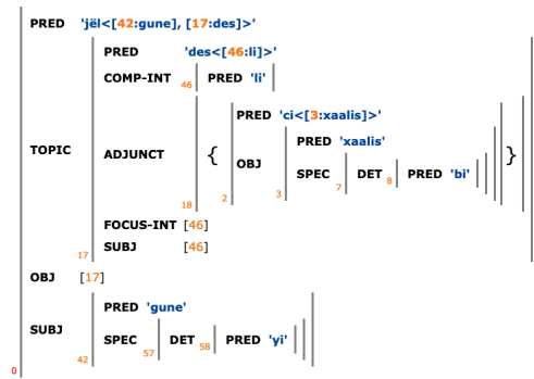
Fig. 10: F-structure of (9)
