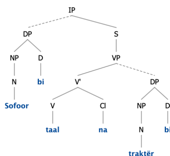
Fig. 1: C-structure of (1)
