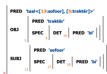
Fig. 2: F-structure of (1)
