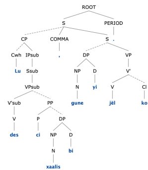
Fig. 9: C-structure of (9)
