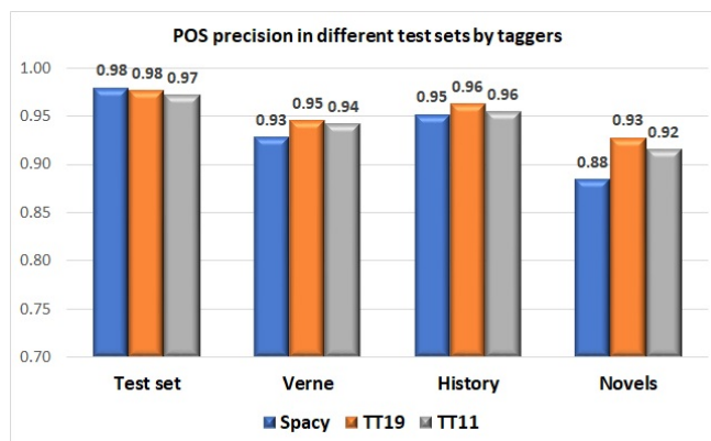
Figure 1: Part-of-Speech tagging accuracy per token on test sets, for each of trained models
