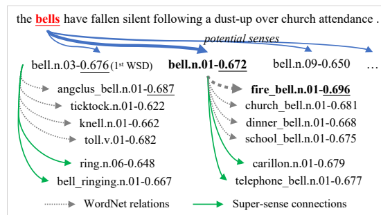
Figure 4: A Test Set Example of the Second WSD
