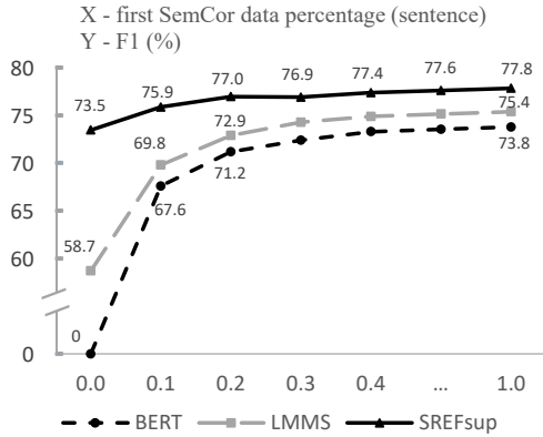
Figure 5: System Performance with Different Proportion of Semcor Sentences
