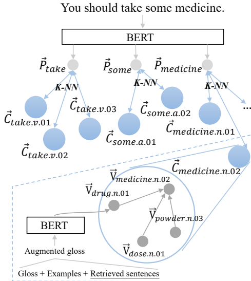
Figure 1: Knowledge-enhanced WSD Framework without the Try-again Mechanism
