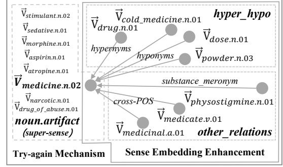
Figure 3: Synset Relation Exploitation for Sense Embedding Enhancement and Try-again Mechanism.
