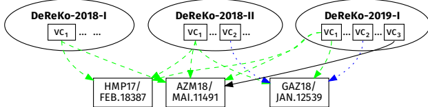
Figure 2 – Visualisation of the relationship between DeReKo releases, virtual sub-corpora and texts. DeReKo contains texts that are not only part of one corpus, but many (virtual) corpora. Considering the versioning, we find that text can be part of many different versions of many corpora.
