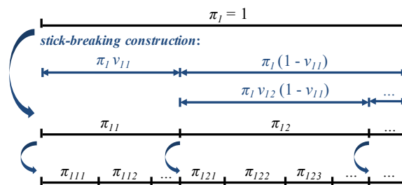
Figure 6: Tree-based stick-breaking construction.
