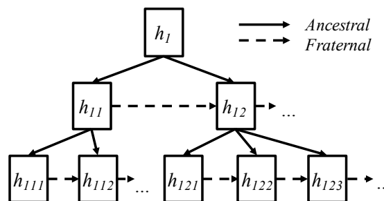
Figure 7: Doubly-recurrent neural networks.
