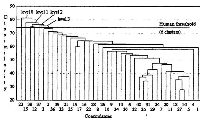
Figure 8: Single-linkage clustering of the keyword 重.. The Human threshold is derived from knowing the number of clusters that human identified and then search the equivalent threshold value that produces the same number of clusters as human (i.e. 6 clusters in this case).
