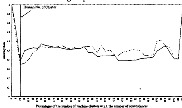
Figure 13: Accuracy of clustering the concordances of the keyword 由 for different numbers of machine cluster. The solid and dotted lines represent accuracy with and without part-of-speech tagging, respectively.
