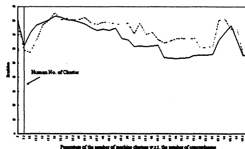
Figure 17: Precision of clustering the concordances of 由 for different numbers of machine cluster. The solid and dotted lines represent accuracy with and without part-of-speech tagging, respectively.
