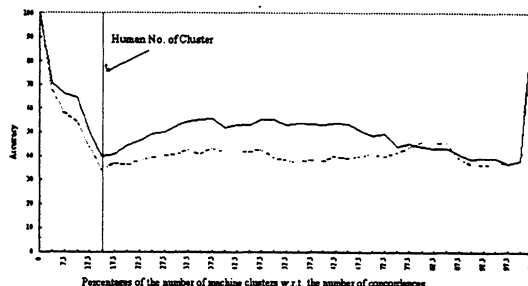
Figure 10: Accuracy performance of the keyword for different numbers of machine cluster. The solid line indicates the performance with part-of-speech tagging and the dotted line without part-of-speech tagging.
