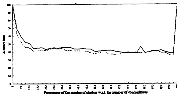
Figure 23: Consistent better accuracy with part-of-speech tagging (solid line) compared with without part-of-speech tagging (dotted line) for different numbers of machine cluster.
