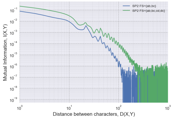
Figure 5: LDD characteristics of datasets of SP2 grammar with varying forbidden subsequences.
