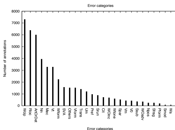
Figure 4: Error categories histogram for the NUCLE corpus.
