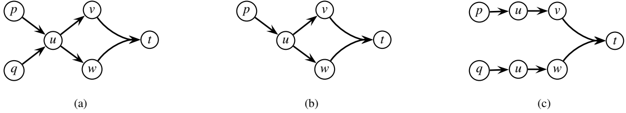
Figure 1: Examples of hypergraph, hyperpath, and derivation: (a) a hypergraph H , with t as the target vertex and p, q as source vertices, (b) a hyperpath \pi_t in H , and (c) a derivation of t in H , where vertex u appears twice with two different (sub-)derivations. This would be impossible in a hyperpath.
