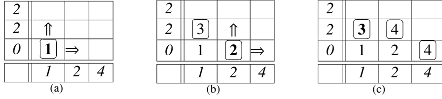
Figure 4: An illustration of Algorithm 1 in |e| = 2 dimensions. Here k = 3 , \leq is the numerical \leq , and the monotonic function f is defined as f(a, b) = a + b . Italic numbers on the x and y axes are a_i 's and b_j 's, respectively. We want to compute the top 3 results from f(a_i, b_j) with 1 \leq i, j \leq 3 . In each iteration the current frontier is shown in oval boxes, with the bold-face denoting the best element among them. That element will be extracted and replaced by its two neighbors ( \uparrow and \Rightarrow ) in the next iteration.
