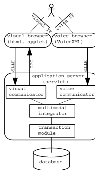
Figure 1: Multimodal Architecture
