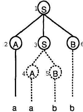
Figure 1: Grammar and parse tree for aabb .
