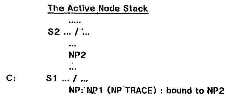
Figure 15 - NP1 must be attached as the subject of S1 since it is bound to an NP Dominated by a higher S.
