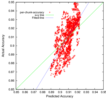
Figure 1: Plot showing Actual vs. Predicted accuracies for WSJ-test (100-sentence chunks). Each plot point represents a 100-sentence chunk. ( rms error = 0.015 )
