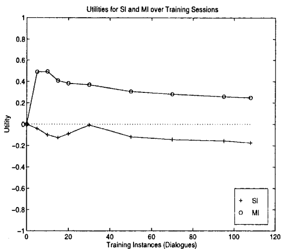
Figure 1: Results of applying Q-learning to System-Initiative (SI) and Mixed-Initiative (MI) Strategies for 108 ELVIS Dialogues
