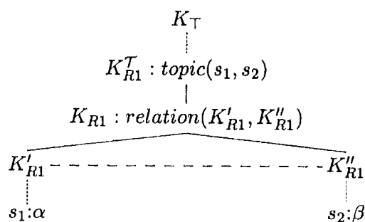
Figure 5: Underspecified discourse structure
