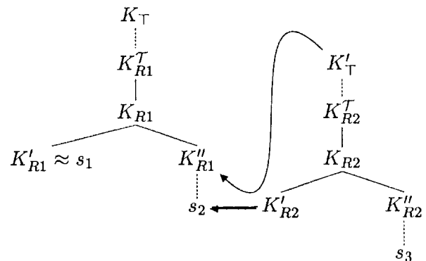
Figure 4: Two tree descriptions combined
