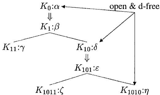
Figure 1: Openness and D-Freedom
