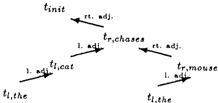
Figure 4: With both left and right adjunctions possible, the sentences can be parsed in a more linguistically plausible way
