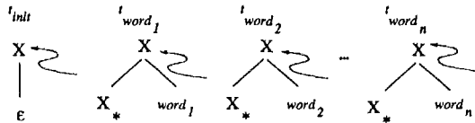
Figure 1: A set of elementary LTIG trees that represent a bigram grammar. The arrows indicate adjunction sites.
