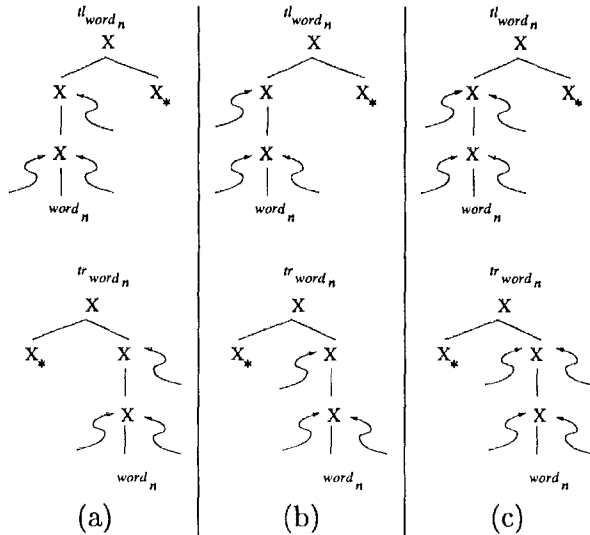
Figure 5: Prototypical auxiliary trees for three PLTIGs: (a) L1R2, (b) L2R1, and (c) L2R2.
