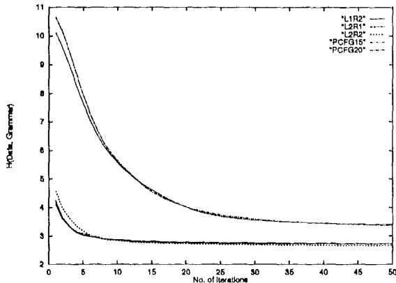
Figure 6: Average convergence rates of the training process for 3 PLTIGs and 2 PCFGs.
