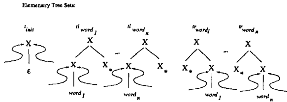
Figure 3: An LTIG elementary tree set that allow both left and right adjunctions.
