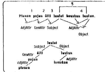
b) A non-monotonous dependency tree
