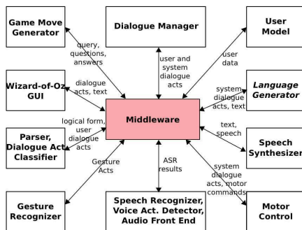
Figure 3: High-level architecture of the integrated system.
