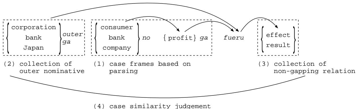
Figure 1: Outline of our method
