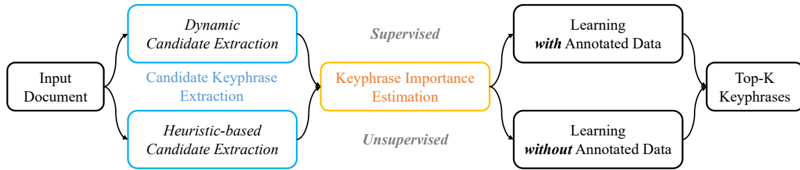
Figure 1: The overall architecture of the two-stage supervised and unsupervised keyphrase extraction framework.
