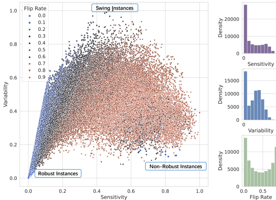
Figure 7: Data map for the AGNEWS train set, based on a BERT-base model. Density plots for the three different measures (sensitivity, variability and flip rate) based on the adversarial loss of each instance during training are shown towards the right. The training instances can be roughly classified into three types: robust instances, non-robust instances and swing instances.
