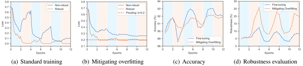
Figure 5: Synthetic continuous learning settings for SST-2. The background color of each column indicates the training partition, with the light blue background denoting training non-robust instances and the light orange denoting training robust instances. The curves in (a) and (b) track the performance of the two partitions during interleaved training, and curves in (c) and (d) indicate the performance of the test set. The figure highlights that mitigating the overfitting of the model to robust instances can reduce the conflict between robust and non-robust instances, making the robust instances to better improve the robustness of the model.
