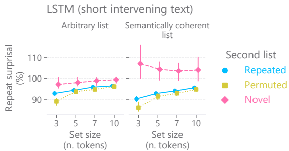
Figure 6: LSTM verbatim token retrieval for varying number of tokens being retrieved at short (4-token) intervening text. Reported is proportion of list-averaged surprisal on second relative to first list of nouns (repeat surprisal). Points show group median (over N^{list} = 230 ). Error bars denote 95% confidence interval around the median (bootstrap estimate).
