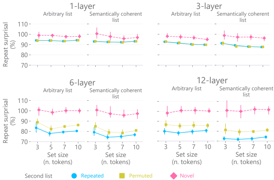
Figure 5: LM memory retrieval for models of different sizes. Reported is relative list-averaged surprisal over all non-initial tokens in lists. Points show group median (over N^{list} = 230 ). Error bars denote 95% confidence interval around the median (bootstrap estimate). Note that in these plots y-axis starts at 70%.
