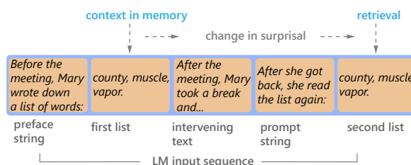
Figure 1: Characterizing verbatim memory retrieval in neural language models. In our paradigm, language models processed English text in which a list of nouns occurred twice. We operationalized retrieval as the reduction in surprisal from the first to the second list presentation. We measured retrieval while varying: a) set size, b) the structure of the second list, c) the length of the intervening text, and d) the content and structure of the intervening text.
