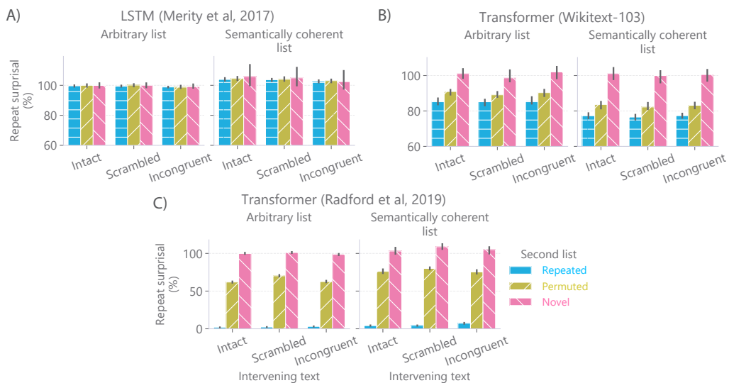
Figure 4: LM memory retrieval for different intervening texts. We plot relative list-averaged surprisal over all non-initial tokens in lists. Points show group median (over N^{list} = 230 ). Error bars denote 95% confidence interval around the median (bootstrap estimate). Note that in the top-row plots y-axis starts at 60%.
