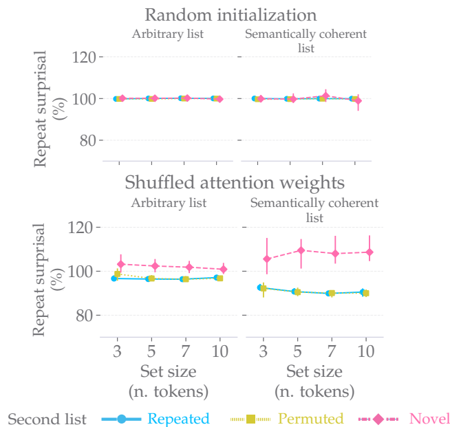
Figure 8: Repeat surprisal for randomly initialized transformer LM and a transformer with permuted attention weights. Reported is relative list-averaged surprisal over all non-initial tokens in lists only. Points show group median (over N^{list} = 230 ). Error bars denote 95% confidence interval around the median (bootstrap estimate). Note that in these plots y-axis starts at 70%.
