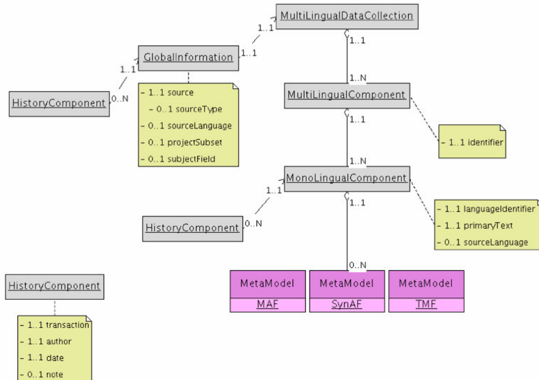
Figure 2. MLIF Metamodel and related Data Categories
