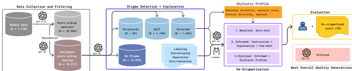
Figure 1: Full stigma extraction and de-stigmatization pipeline.
