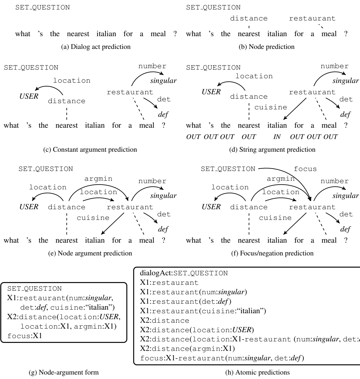
Figure 2: Semantic parsing decomposition.
