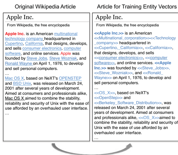
Figure 2: Training entity vectors from anchor texts.
