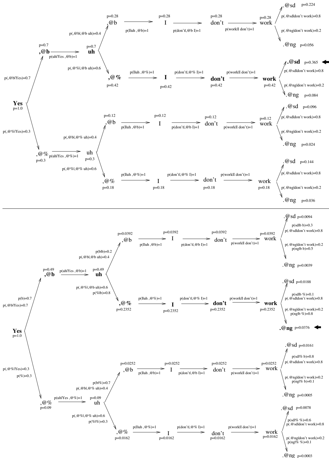
Figure 3: An example of the Viterbi tree search for the basic NGT model (top) and for the enhanced NGT model (bottom). In the basic model only the NGT probabilities are taken into account. In contrast, in the enhanced model both the NGT probabilities and the DA language model probabilities are used in the transitions where outputs are produced. In these nodes, the new probability is the result of multiplying the probabilities of the parent node, the NGT probability and the DA language model probability. Best hypothesis (in boldface and marked by the dark arrow) changes from (b % sd) to (b % ng). In this example, trigrams are used in all models.
