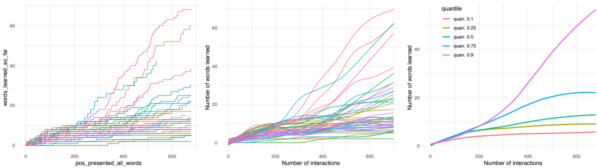
Figure 6: Plots of empirical growth trajectories (left), predicted growth trajectories from cubic model (center), and average predicted vocabulary growth at the 10th, 25th, 50th, 75th, and 90th percentiles.
