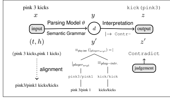
Figure 7: The prediction model: input is mapped to a hidden derivation d using a PCFG (parameterized by \theta ), which is then used to generate an output semantic representation. In the case of semantic parsing (top), d is a latent semantic parse tree and the output is a logical representation. For entailment detection, d is a latent proof tree and the output is a human judgement about entailment.
