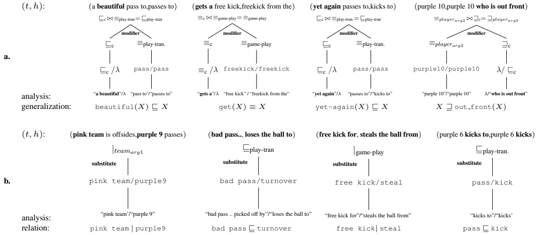
Figure 9: Example construction-based (a) and lexical-based (b) inferences (both defined in Section 2.2) taken from parts of proof trees learned during our experiments. While inferences are computed between semantic concept symbols (e.g., purple4 , pass , ≡c ), the generalizations in a. show how such structures can be used to generate lexicalized inference rules.
