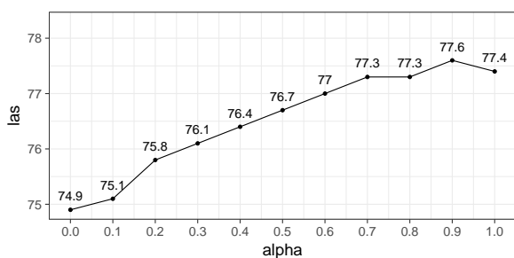
Figure 5: The effect of \alpha on distillation.
