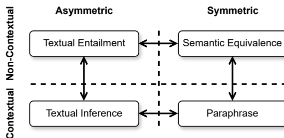
Figure 1: Four sentence-level relations in terms of symmetry and contextuality. Arrows indicate interdependence between the relations (Section 2).
