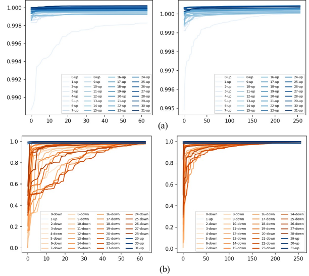
Figure 7: Normalized similarity between quantization error and subspaces spanned by singular vectors of learned adapter per layer. (a) Query projection (b) Up protection, Left: U_{A_r=64} B_{r=64} Right: U_{A_r=256} B_{r=256} LLaMA-2-7b wikitext fine-tuning.
