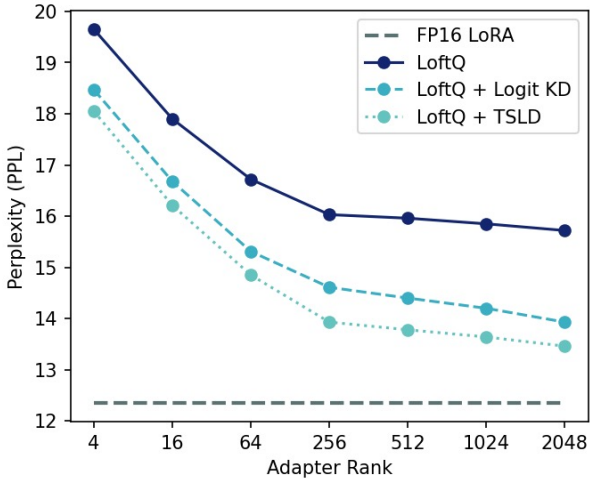
Figure 10: OPT-1.3b WikiText-2 LoftQ PPL results with Knowledge Distillation methods with adapter rank exploration. Logit KD denotes conventional logit distillation and TSLD denotes Token-Scaled Logit Distillation (Kim et al., 2023) KD method for decoder-only model.
