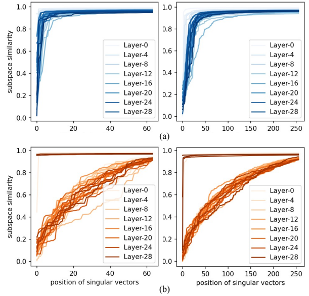
Figure 3: Normalized similarity between quantization error and subspaces spanned by singular vectors of learned adapter per layer. (a) Query projection (b) Up-Projection, Left: U_{AB_{r=64}} Right: U_{AB_{r=256}} 2-bit quantization-aware GSM8K fine-tuned LLaMA-2-7B model is used for analysis.
