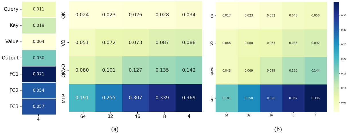
Figure 9: Fine-tuning performance ablation study across various ranks. Each cell represents the performance degradation when adjusting the rank of specific sub-layers, as indicated on the x-axis during LLaMA-2-7B Fine-Tuning on WikiText-2 with rank 256. (a) LoftQ (Li et al., 2024) ( r = 256 PPL: 6.8427) (b) LQ-LoRA (Guo et al., 2024) ( r = 256 PPL: 6.6939)
