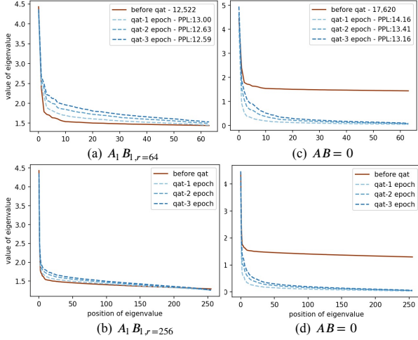
Figure 6: Singular values of low-rank adapters across fine-tuning epochs with PPL performance. (a),(b) fine-tuning LoftQ-1step initialization. rank 64 and 256 respectively (c),(d) AB = 0 rank 64 and 256 respectively. (OPT-1.3B 15th Query layer with Wikitext fine-tuning)
