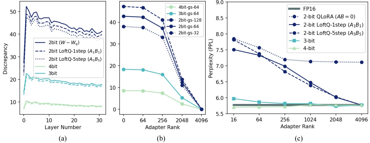
Figure 1: (a) Discrepancy (Frobenius norm) between quantized weight and original pre-trained weight with LoRA adapter with r = 64 . The dashed line represents LoftQ-1step ( A_1B_{1,r=64} ), and the dotted line represents LoftQ-5step ( A_5B_{5,r=64} ). (b) Weight discrepancy comparison by sweeping adapter rank( r ) from 4 to 4096 with LoftQ initialization ( A_5B_{5,r} ). Note that even with fine-grained quantization with group size 32, the trend of requiring a high rank to reduce 2-bit quantized error still exists. (c) LLaMA-2-7B WikiText-2 Quantization-aware LoRA fine-tuning PPL results across QLoRA and LoftQ methods with adapter rank exploration.
