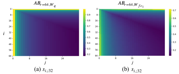
Figure 8: Similarity distance heatmap between W_{qerr} and AB_{r=64} . (a) Query layer (b) FC1 layer. To visualize the differences in color for each element of the heatmap, we truncate the dimension along the j axis to 32.
