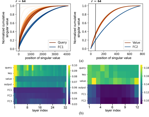
Figure 4: (a) Normalized cumulative singular value of quantization error ( W_{qerr} ) (b) Heat map of normalized cumulative singular value at the 64th singular value. Left: LLaMA-2-7B right: DeBERTa-V3-base
