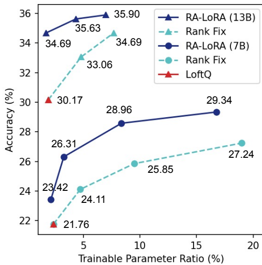
Figure 5: Comparison of 2-bit GSM8K fine-tuning accuracy with LLaMA-2-7B and LLaMA-2-13B across trainable parameter ratios, showcasing RA-LoRA superior accuracy over Rank Fix strategy (Li et al., 2024) (Guo et al., 2024) at all trainable parameter ratios.
