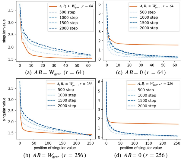
Figure 2: singular values of low-rank adapters across fine-tuning steps. (a),(b) fine-tuning LoftQ-1step initialization. rank 64 and 256 respectively (c)(d) AB = 0 rank 64 and 256 respectively. Note that A_1B_1 in (c) and (d) serve as references. (LLaMA-2-7B Up projection layer with GSM8K fine-tuning)
