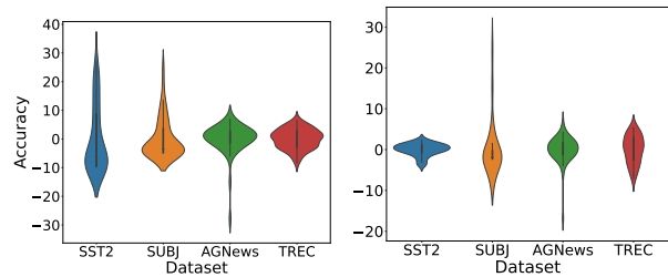
Figure 1: Zero-centered ICL accuracy of 50 random orders on Sheared LLaMA2 1.3B (left) 2023 and LLaMA2 7B (right) 2023.
