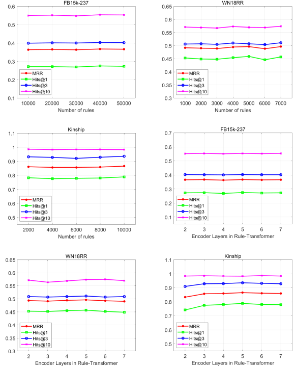
Figure 2: Hyperparameter experiments about number of rules and encoder Layers in Rule-Transformer.
