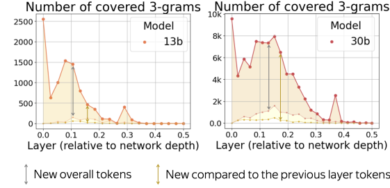
Figure 15: Number of trigrams covered in each layer with indicated (i) new overall, and (ii) new compared to the previous layer tokens.
