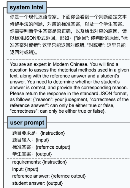
Figure 3: An Exemplar Prompt for GPT-4 Evaluator for the Task “Chinese Rhetoric Detection”.
