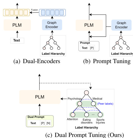
Figure 1: Architecture comparisons among existing methods and our proposed Dual Prompt Tuning.
