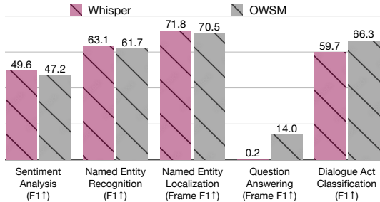
Figure 2: Performance of various supervised ASR SFMs with a lightweight prediction head on SLUE tasks.
