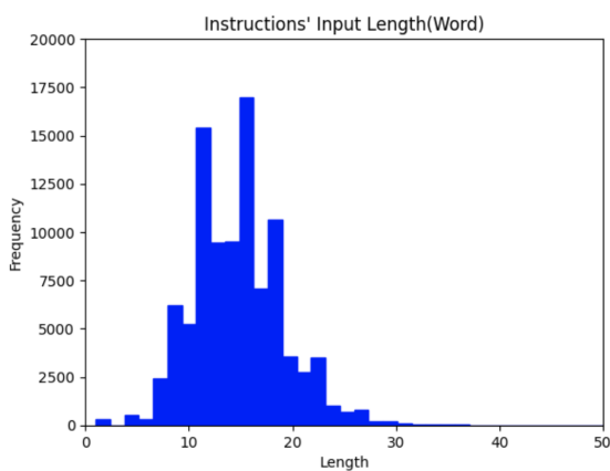
Figure 9: A histogram of Instruction's Input Length distributions
