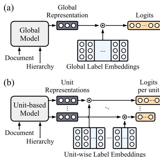
Figure 1: Classification processes of (a) Global and (b) Unit-based HTC models.
