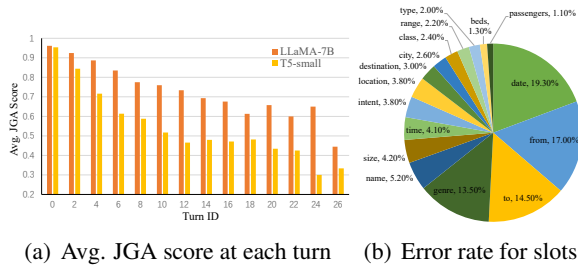
Figure 2: Performance analysis of LLaMA-7B and T5-small in Continual DST task.
