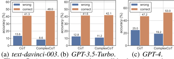
(a) text-davinci-003 . (b) GPT-3.5-Turbo . (c) GPT-4 . Figure 5: Accuracy (averaged over all backward questions across the six data sets) of predicting the masked number in backward questions with correct/wrong candidate answers.
