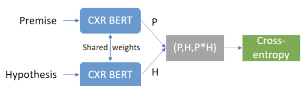
Figure 7: Natural language inference (NLI)
