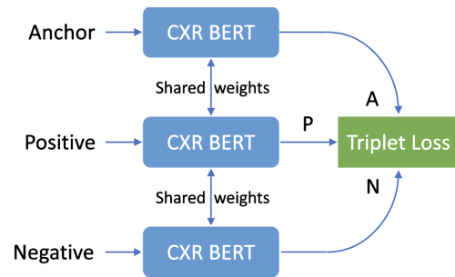
Figure 4: Triplet loss (T)
