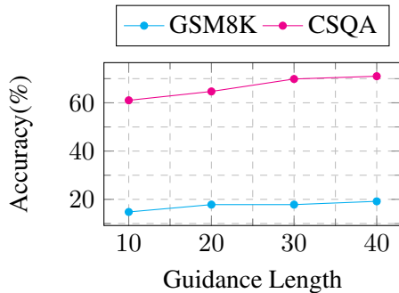
Figure 4: Performance of different length ranges. We use Llama2-13B as teacher model and Llama2-7B as student model.
