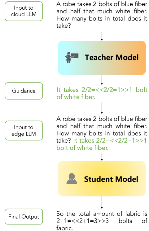
Figure 6: Example for GKT framework
