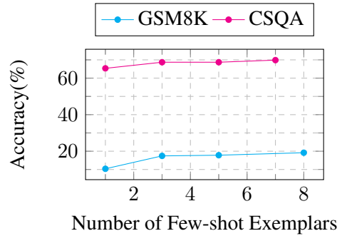
Figure 5: Performance of different few-shot exemplar number
