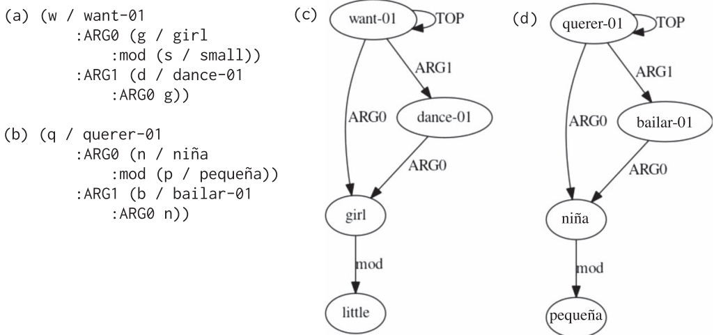
Figure 1 English (a) and Spanish (b) AMRs for the sentence “the little girl wants to dance” la niña pequeña quiere bailar in PENMAN (text-based) notation (Wein et al. 2022a), as well as the English (c) and Spanish (d) graph-based AMR illustrations.
