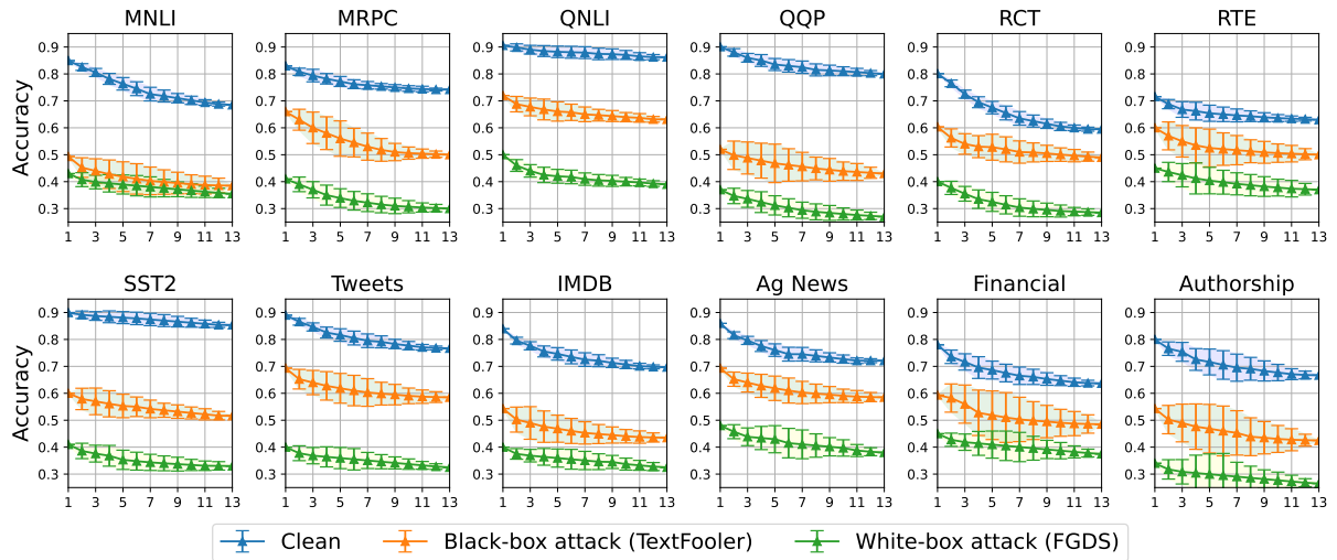
Figure 12: Performance Evaluation of BERT Using the Houlsby (Houlsby et al., 2019) across Varied Domain Datasets.
