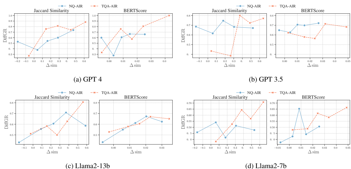
Figure 15: The generation ratio in slices with different average \Delta \text{sim} . \Delta \text{sim} is the difference in similarity between the generated context and the retrieved context. The LLM marked in the figure serves both as a generator and a reader.
