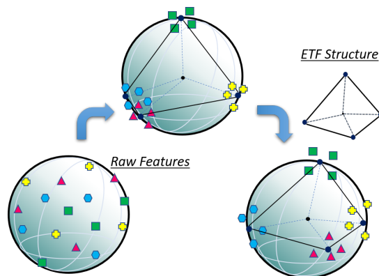
Figure 1: Illustration for the effect of our off-line ETF structure: Having gotten suboptimal features from the simple similarity-based method, we achieve an optimal feature distribution structure by bringing the samples closer to a fixed ETF structure.
