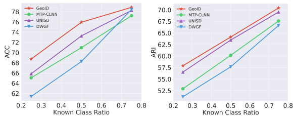
Figure 4: Comparisons on BANKING with varying known class ratios ranging from 0.25 to 0.75.
