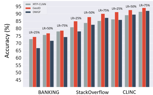
Figure 7: Accuracy comparison with different labeled ratios on different dataset.
