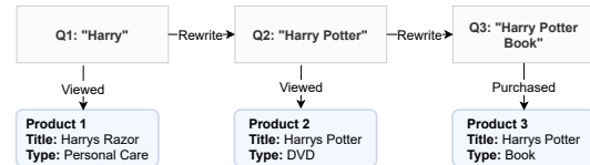
Figure 1: Illustration of a customer session. A session consists of two types of items: queries and products. The customer searched for 3 keywords sequentially and interacted with the products returned by the search engine.
