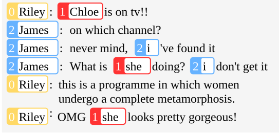
Figure 3: One dialogue example with labeled coreference clusters: there are three coreference clusters in this conversation, where each cluster contains all mentions of one personal identity.
